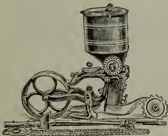
Hill and Drill Seeder Attachment
